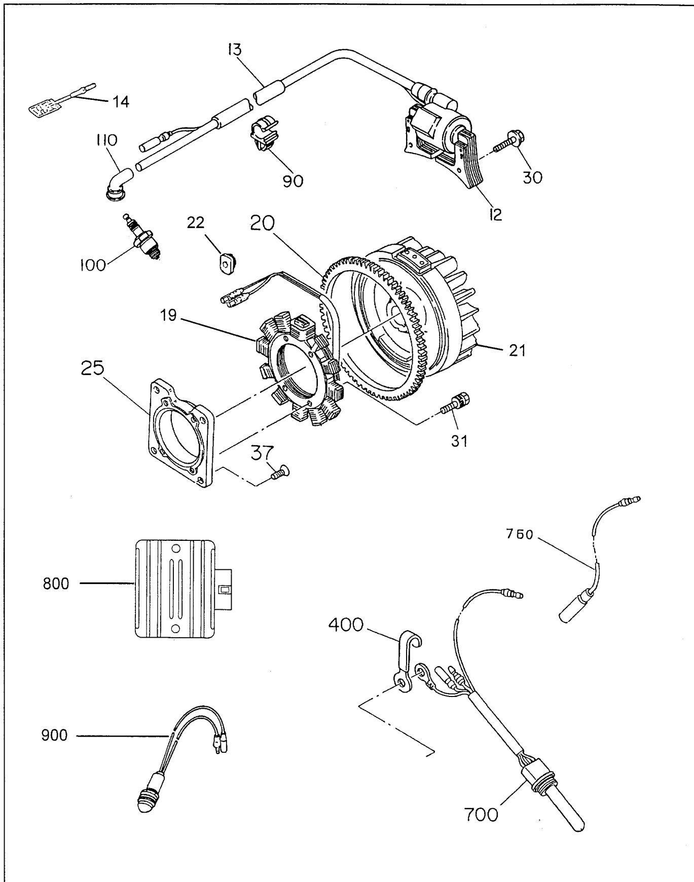
FIG. 7 ELECTRICAL GROUP
