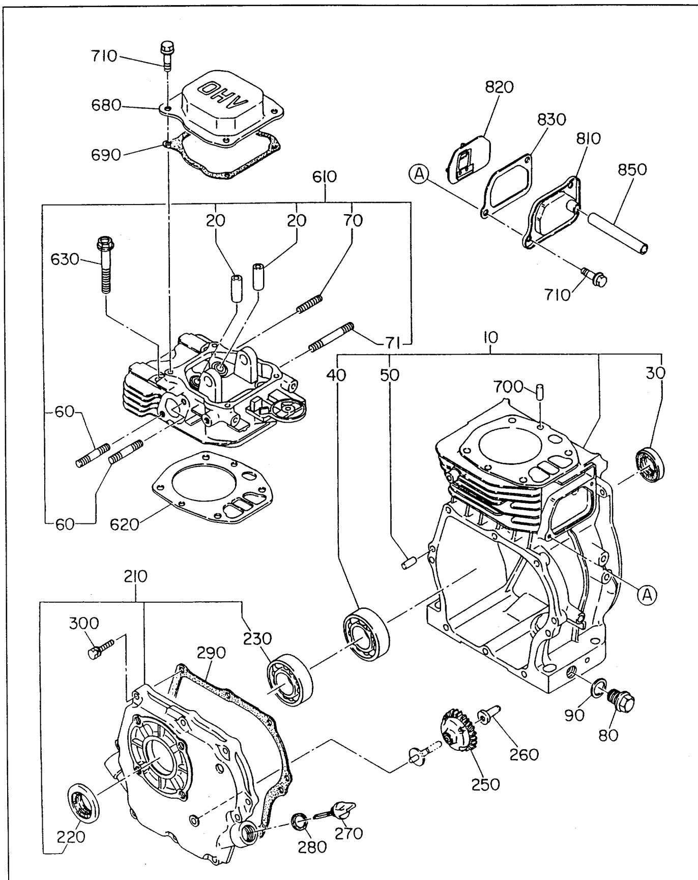
FIG. 1 CRANKCASE GROUP
