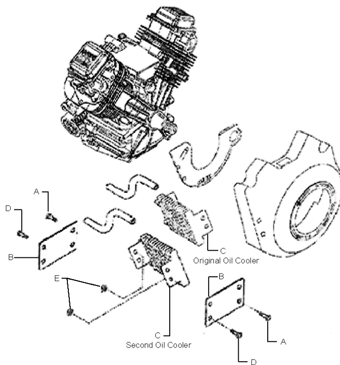
DUAL OIL COOLER 99657740
