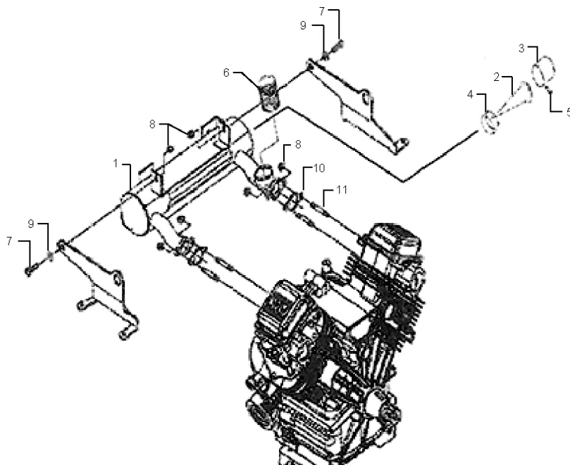
MUFFLER KIT LEFT HAND STARTER SIDE DISCHAGE 99657710
