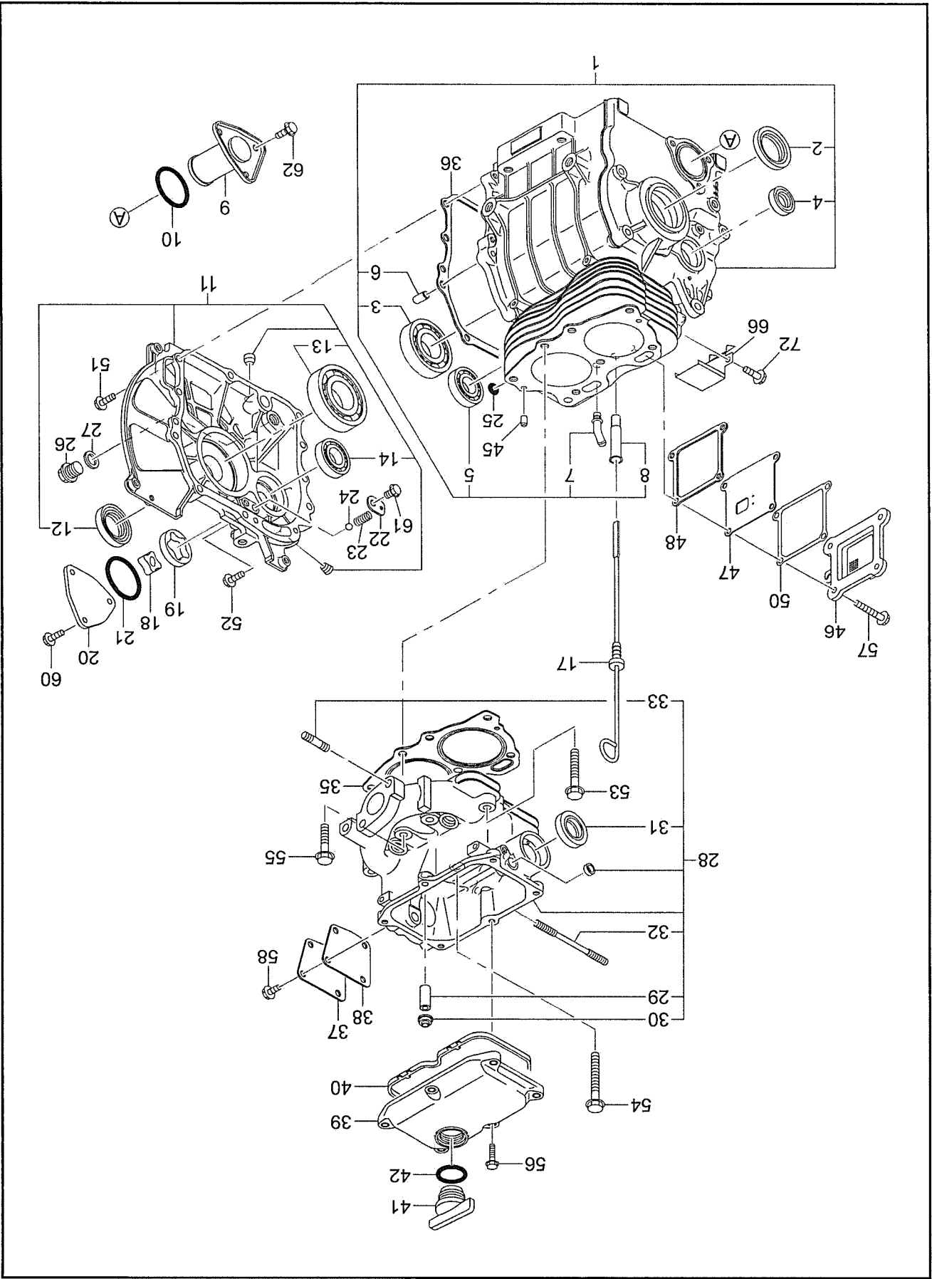
FIG.1 CRANKCASE and CYLINDER
