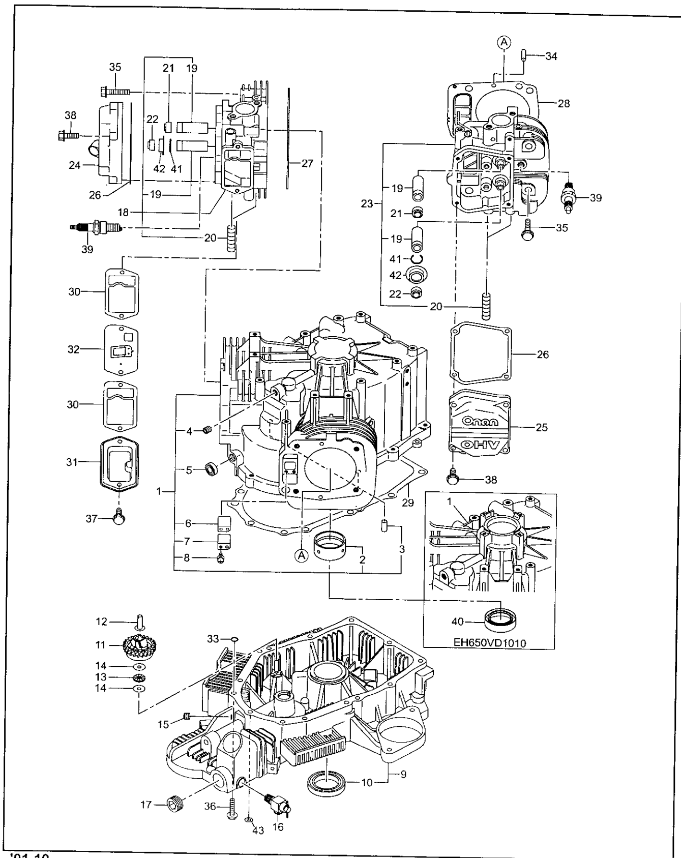
FIG.1 CRANKCASE GROUP
