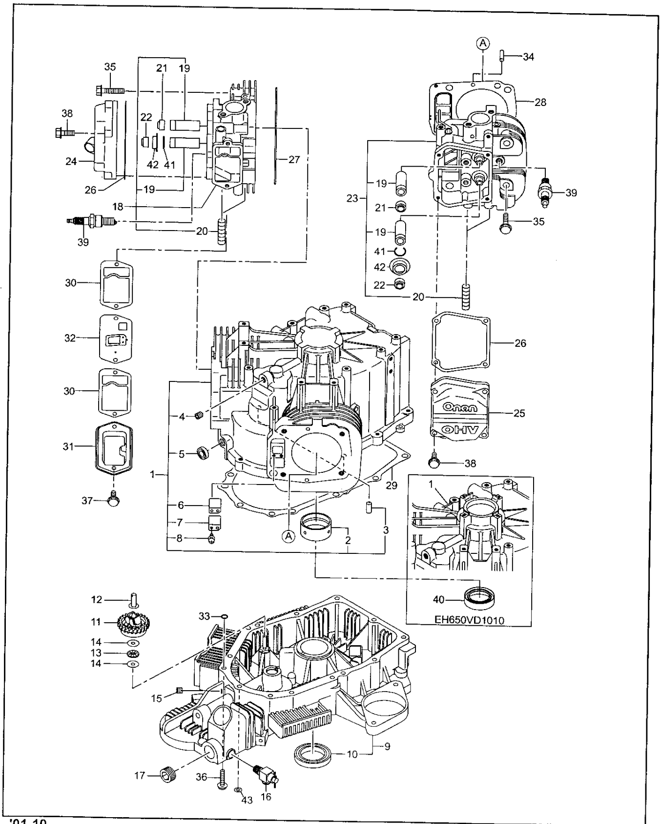
FIG.1 CRANKCASE GROUP
