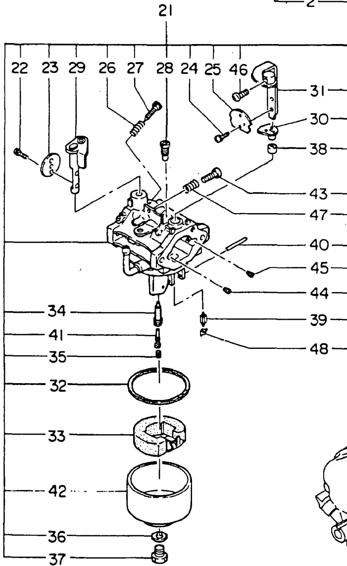
DETAIL "B"
