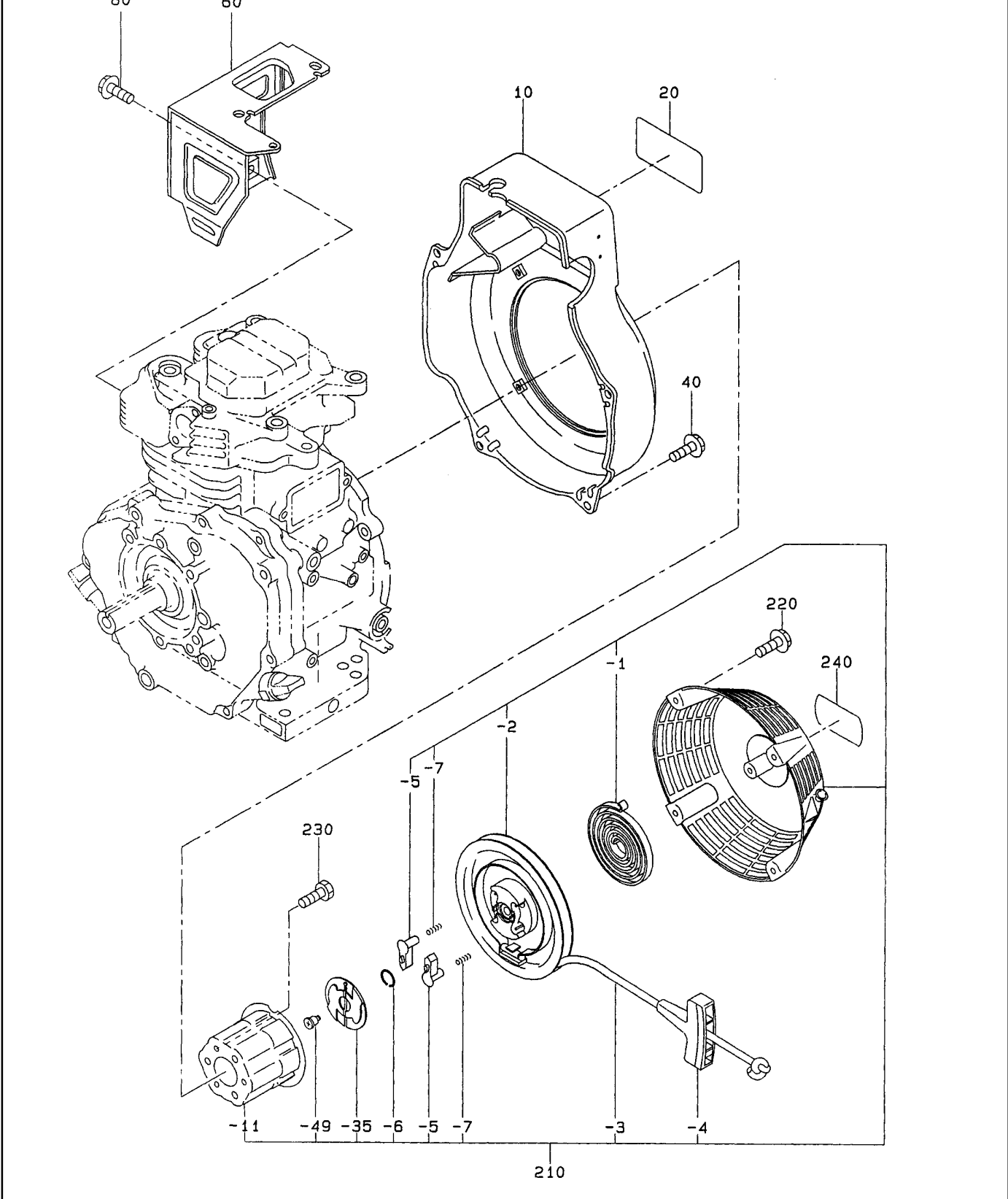
NEW STYLE RECOIL
