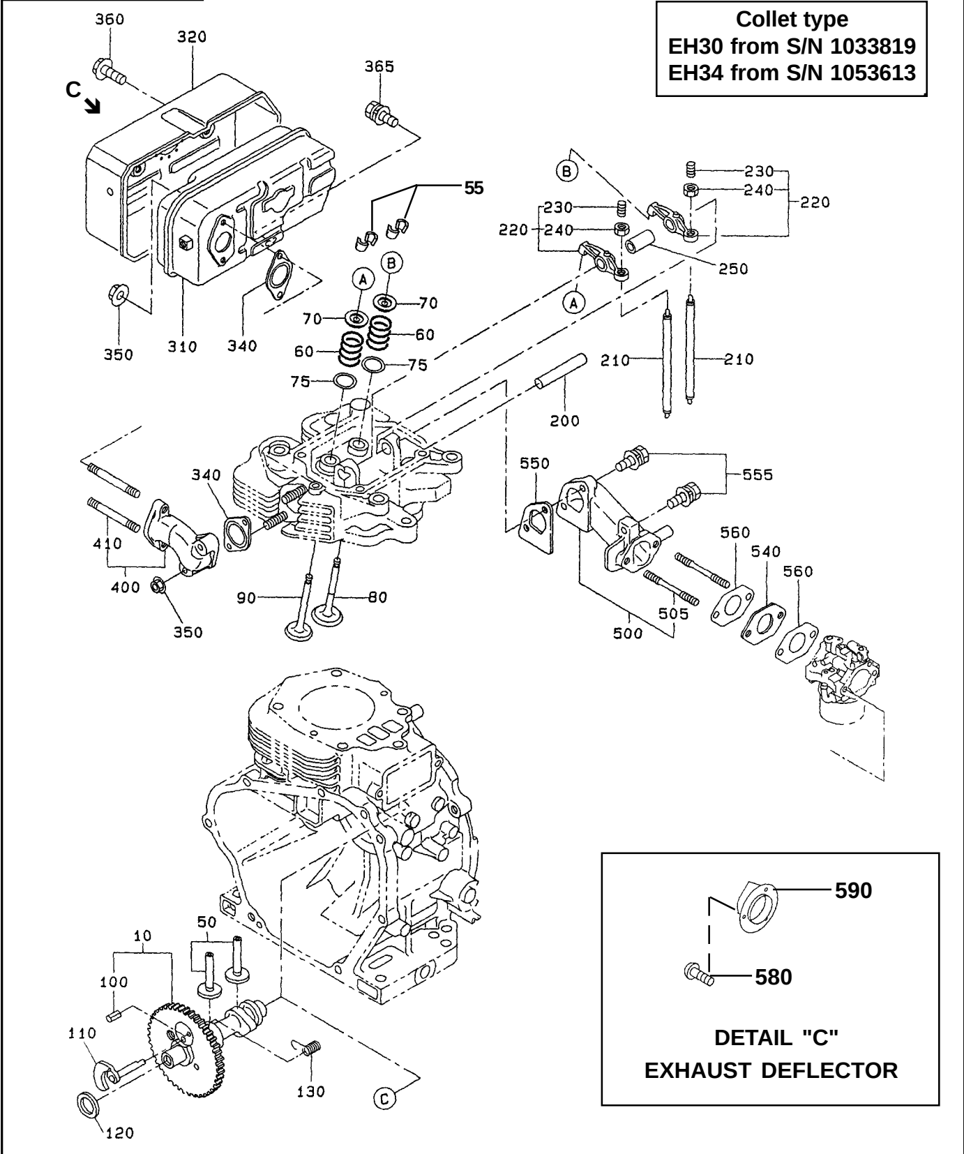
FIG. 300 NEW STYLE VALVE RETAINER
