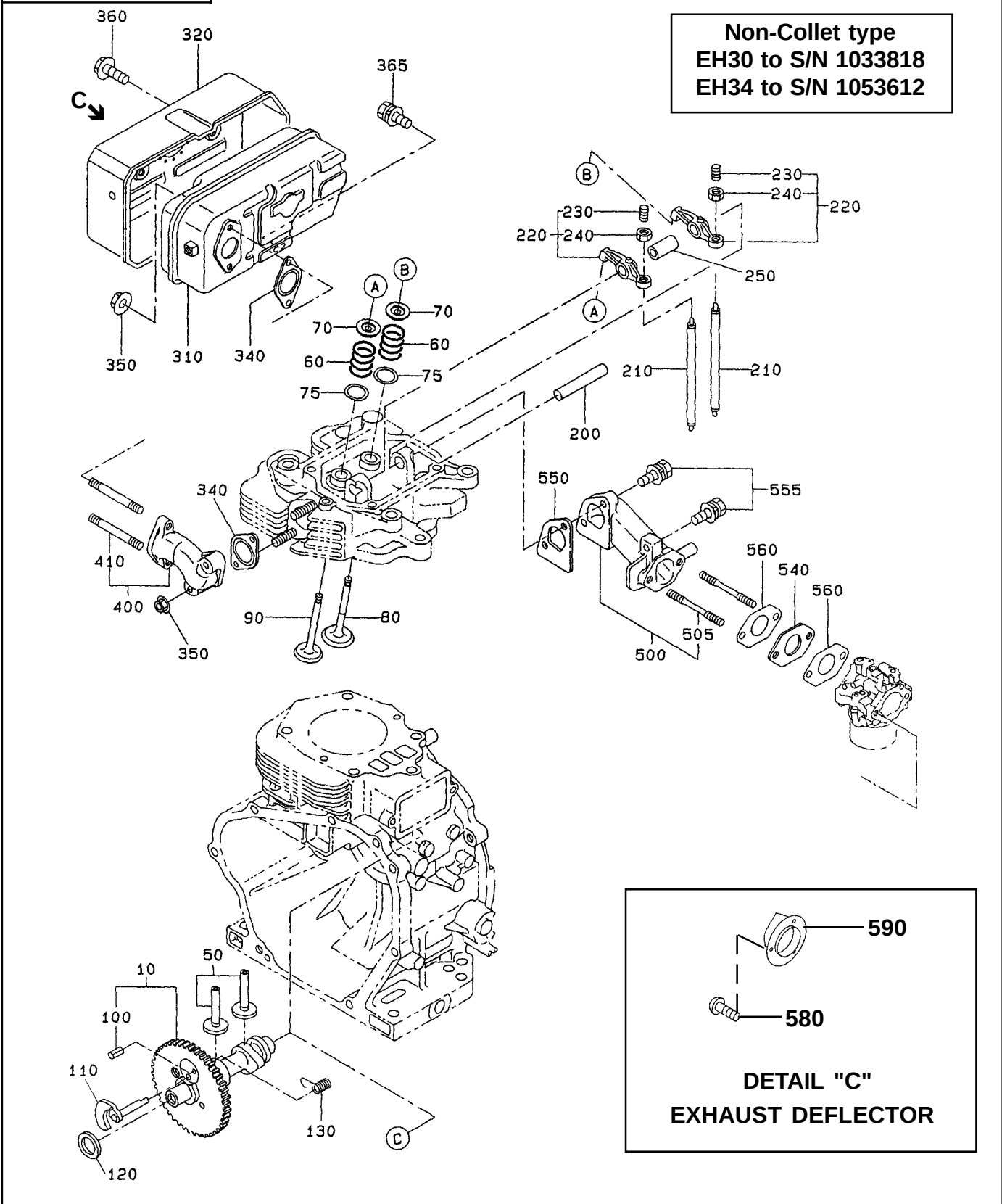
FIG. 310 OLD STYLE VALVE RETAINER
