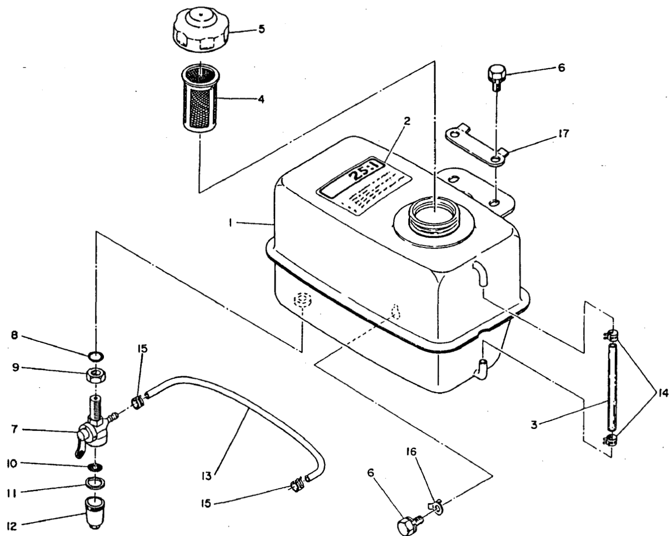
1. FUEL TANK
