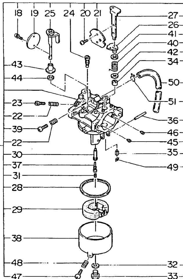
DETAIL "A"
