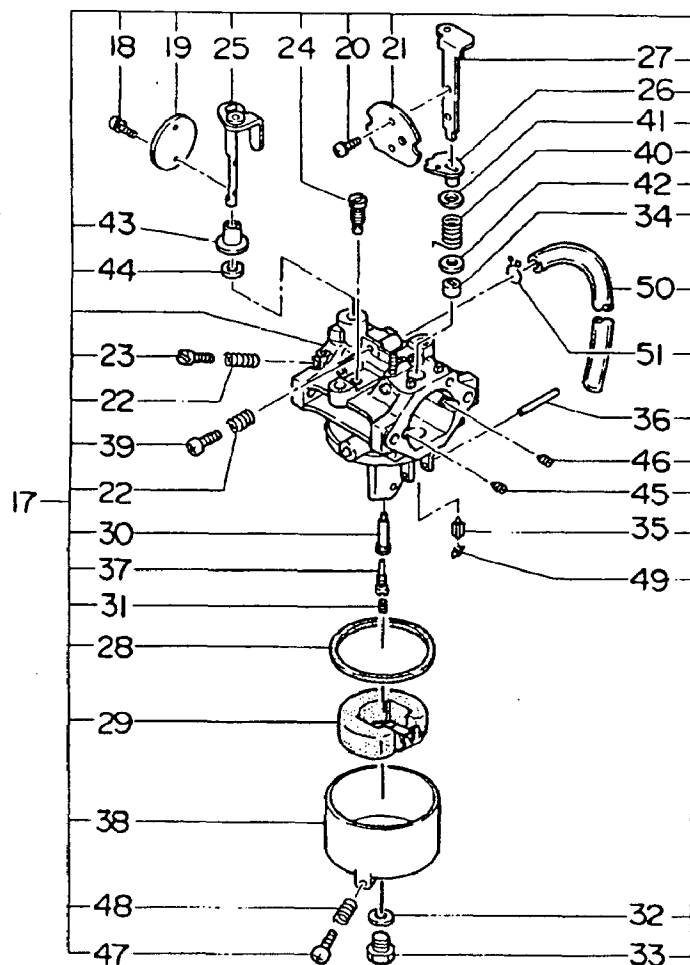
DETAIL "A"
