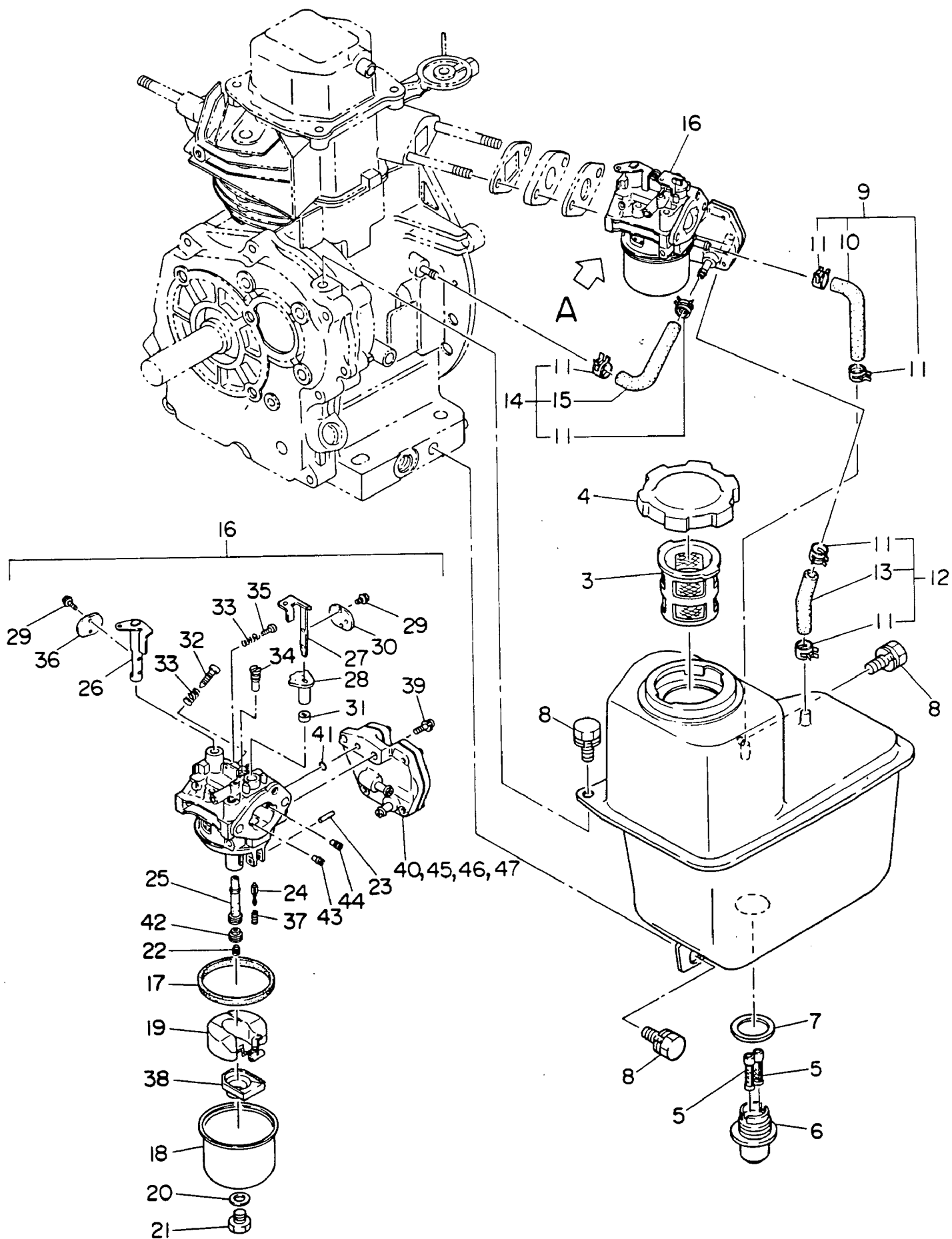
DETAIL "A"
