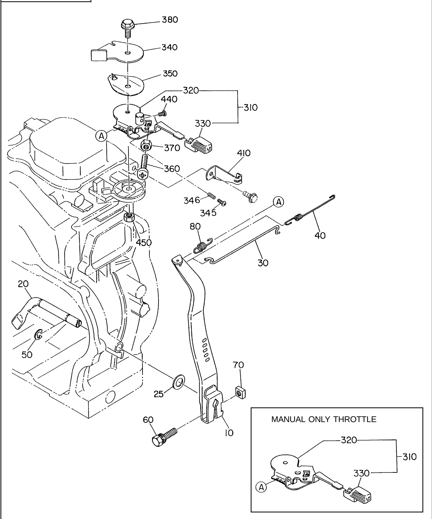
FIG. 400 MANUAL THROTTLE CONTROL with REMOTE CABLE OPTION
