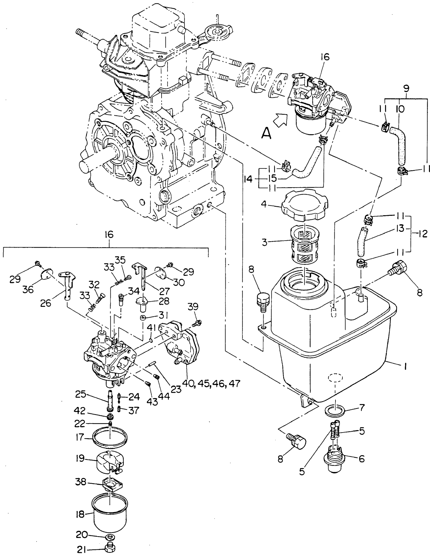
DETAIL "A"
