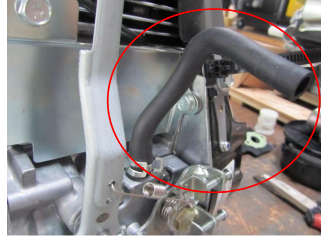
6. Exchange to Breather pipe for float carburetor
