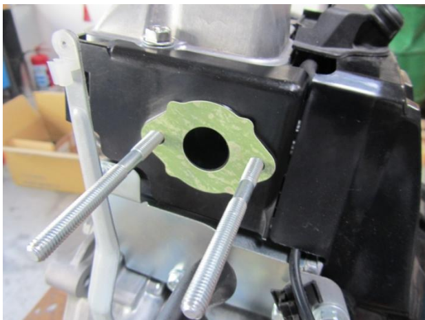
11. Assemble Gasket for float carburetor
