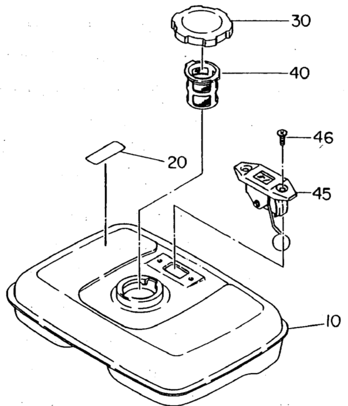
W/FLOAT GAUGE
