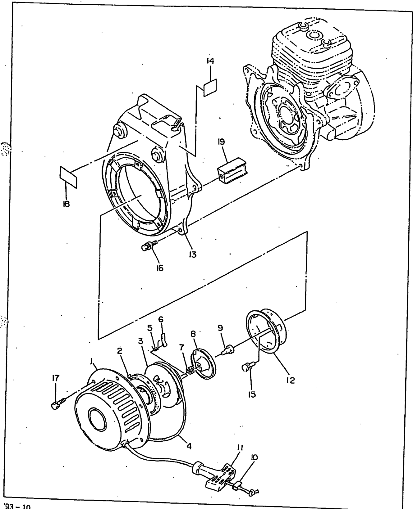
FIG. 4 RECOIL STARTER and BLOWER HOUSING
