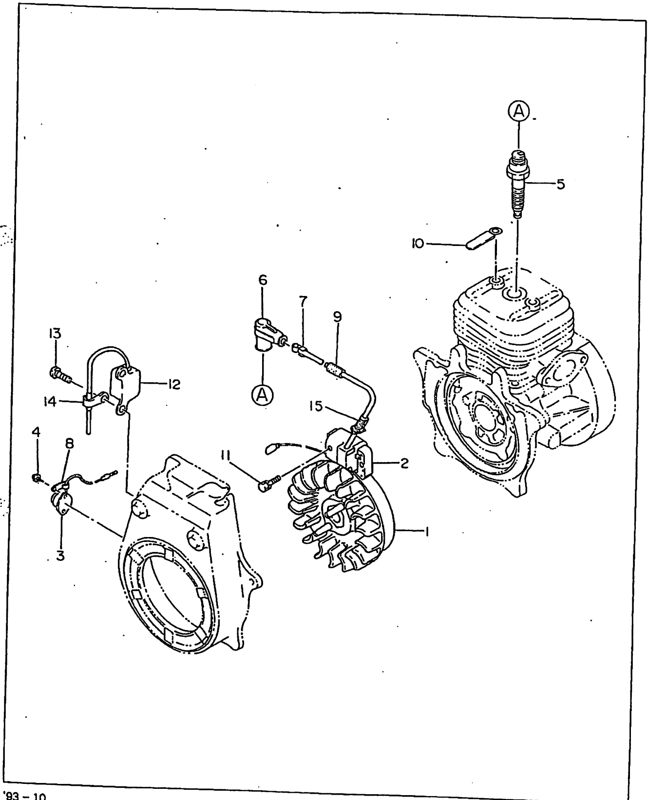
FIG. 6 ELECTRIC DEVICE
