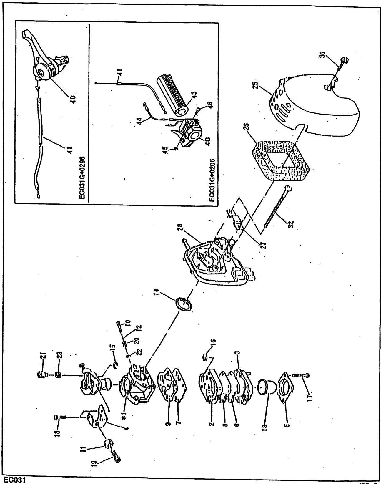
FIG.2 CARBURETOR and CLEANER AIR
