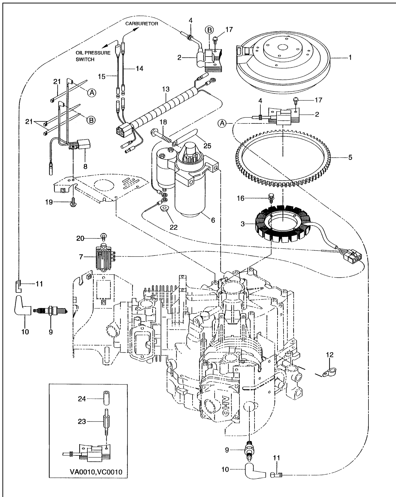
FIG. 9 ELECTRIC DEVICE GROUP - EH63V / EH65V
