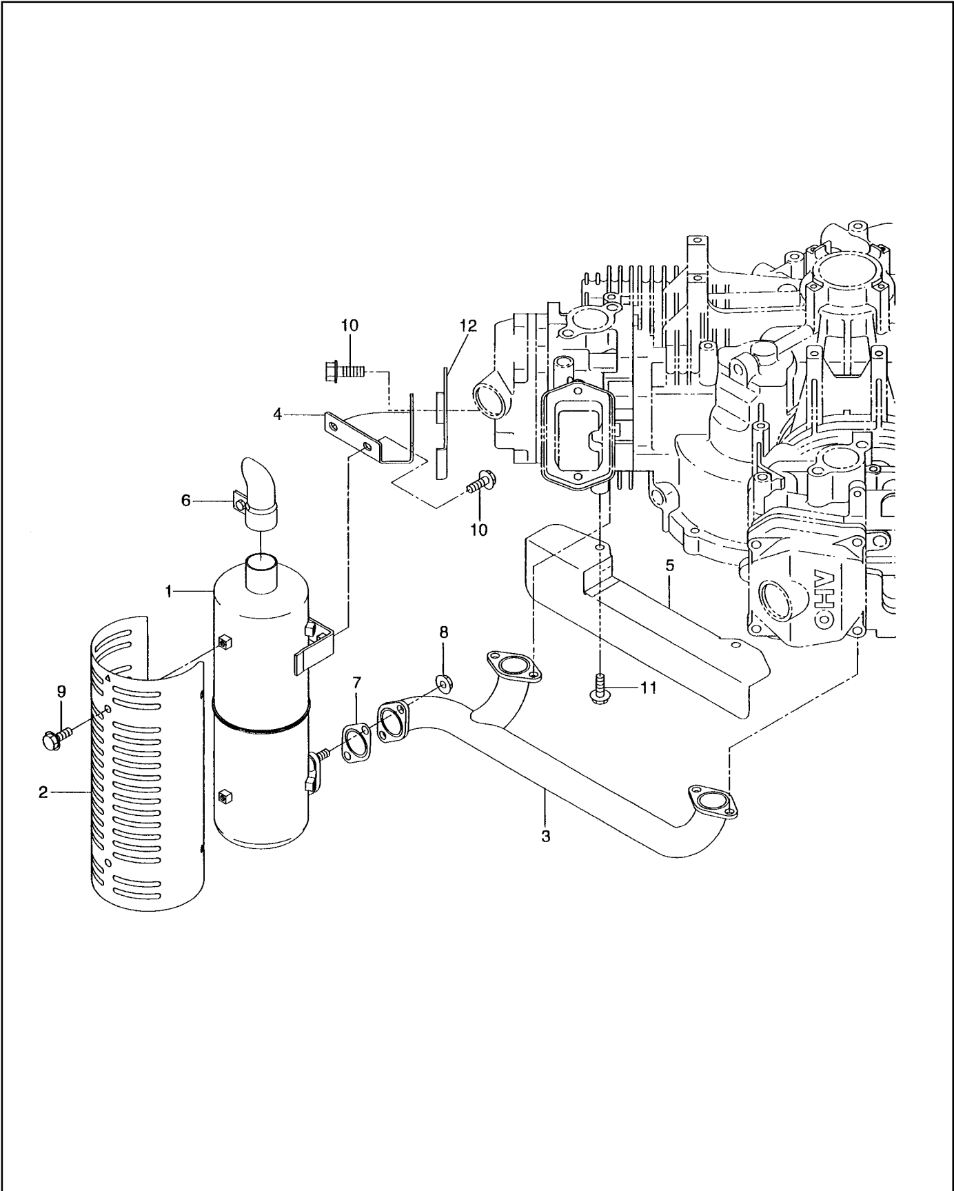
FIG. 4 MUFFLER GROUP (OPTION PARTS) - EH63V / EH65V
