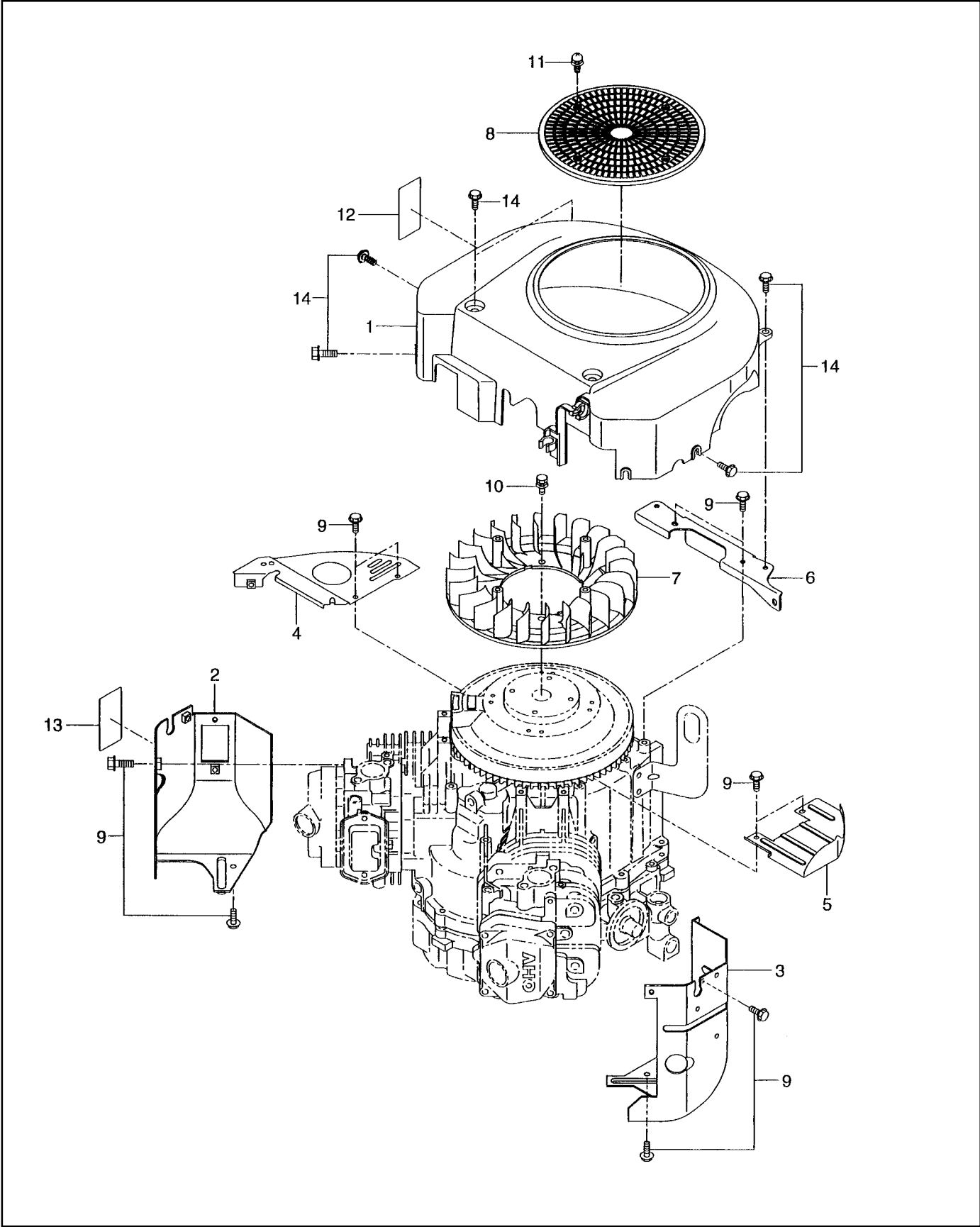
FIG. 6 COOLING and STARTING GROUP - EH63V / EH65V
