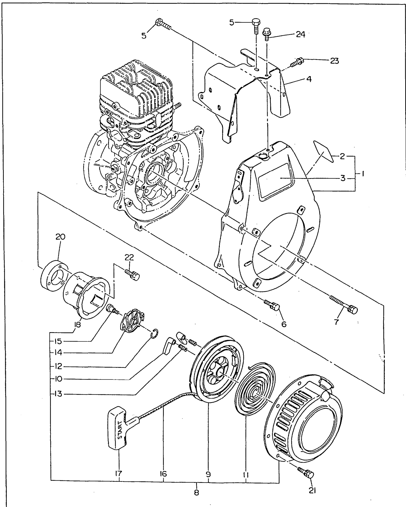
FIG. 4 BLOWER HOUSING and RECOIL STARTER
