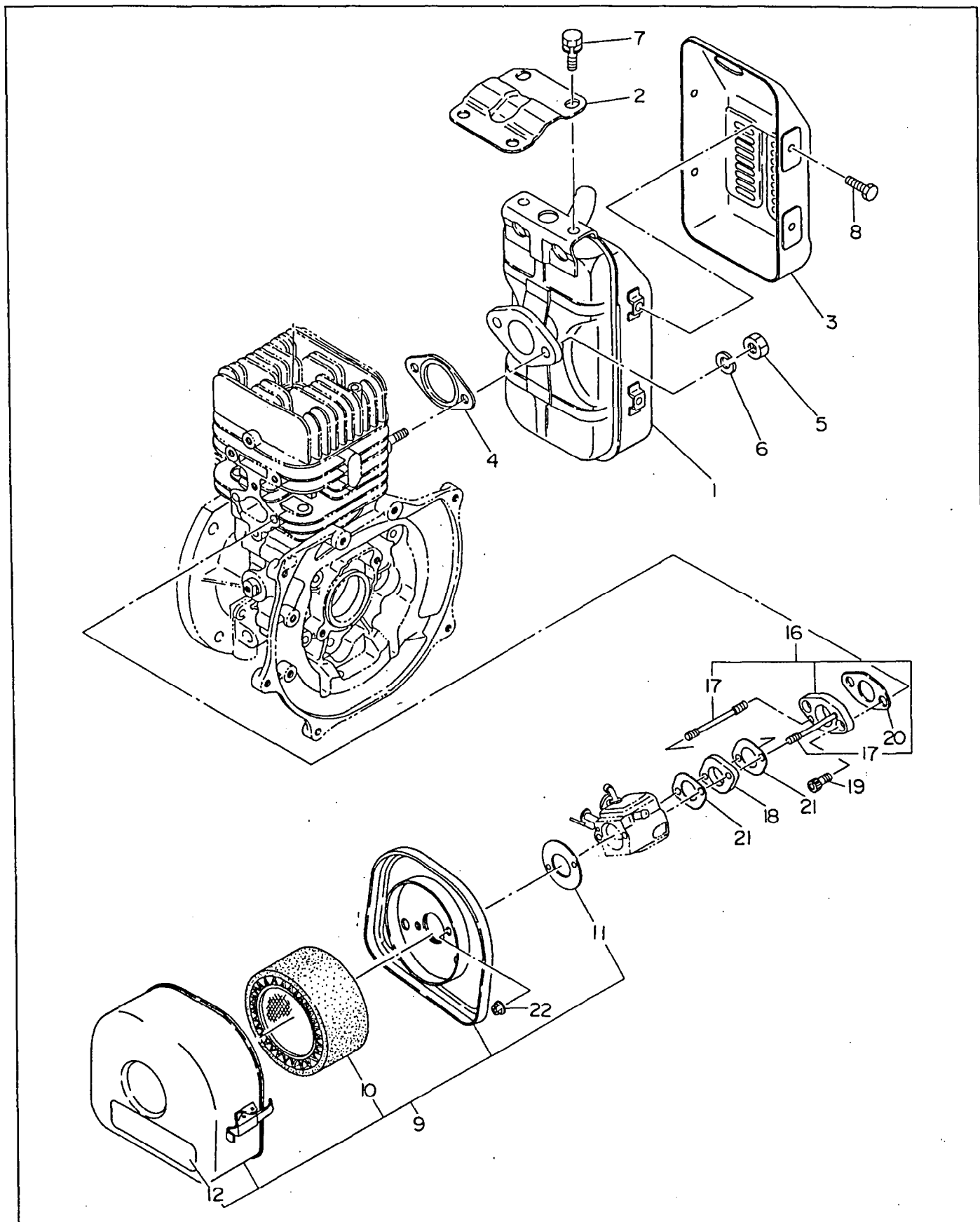
FIG. 3 MUFFLER and AIR CLEANER
