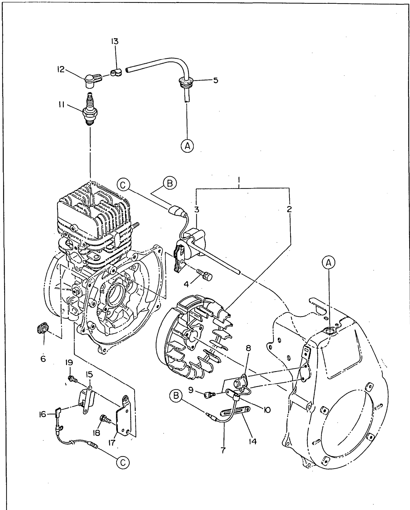
FIG. 6 ELECTRIC DEVICE
