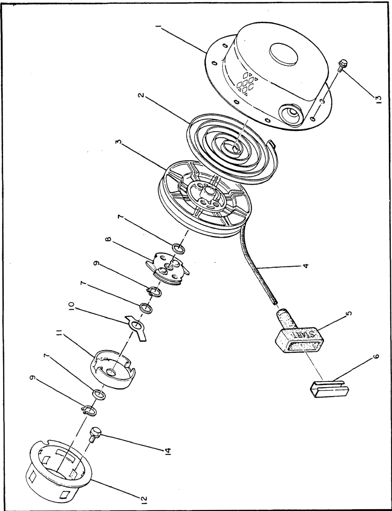
RECOIL STARTER
