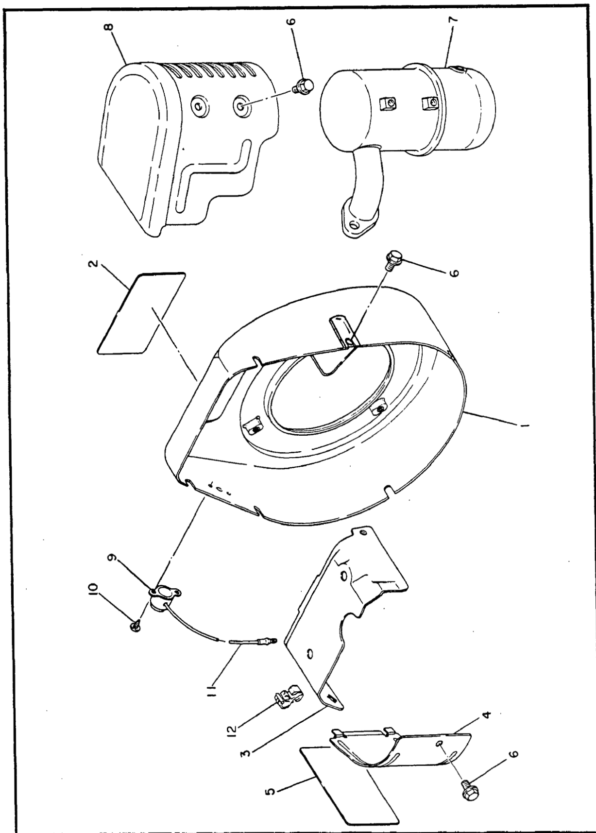
BLOWER HOUSING, STARTING PULLEY AND MUFFLER
