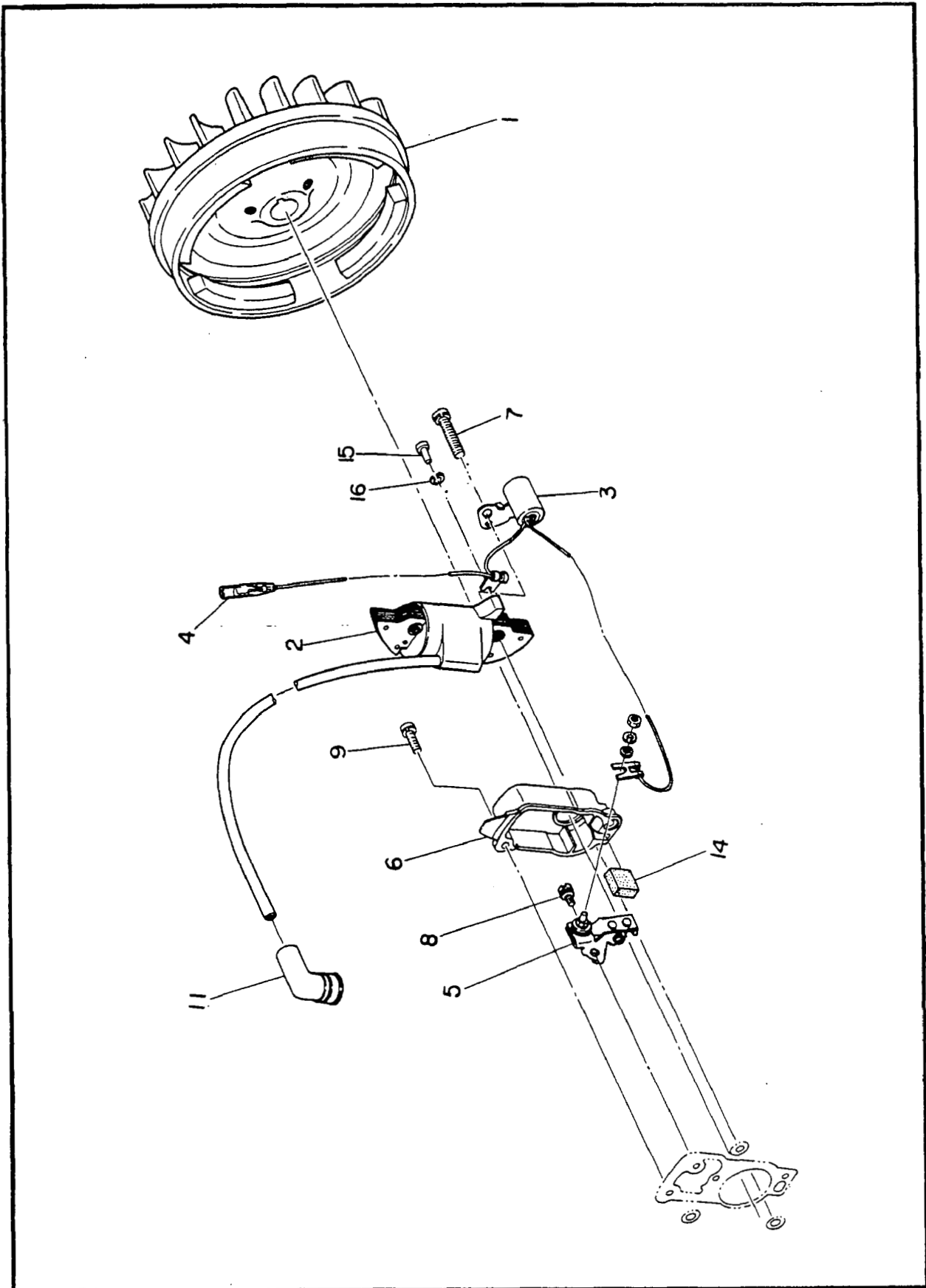
MAGNETO, FLYWHEEL AND IGNITION SYSTEM
