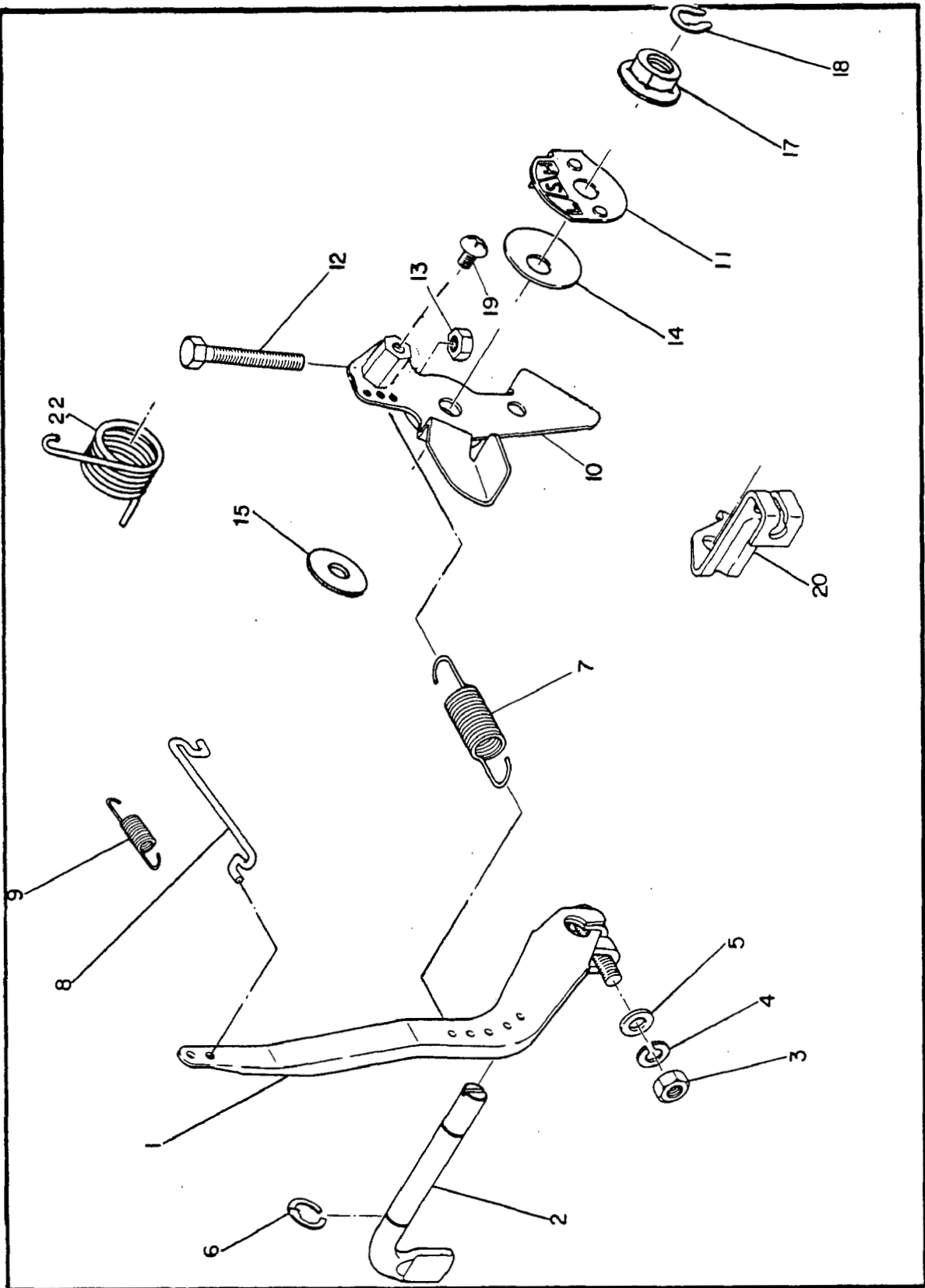
GOVERNOR ASSY.
