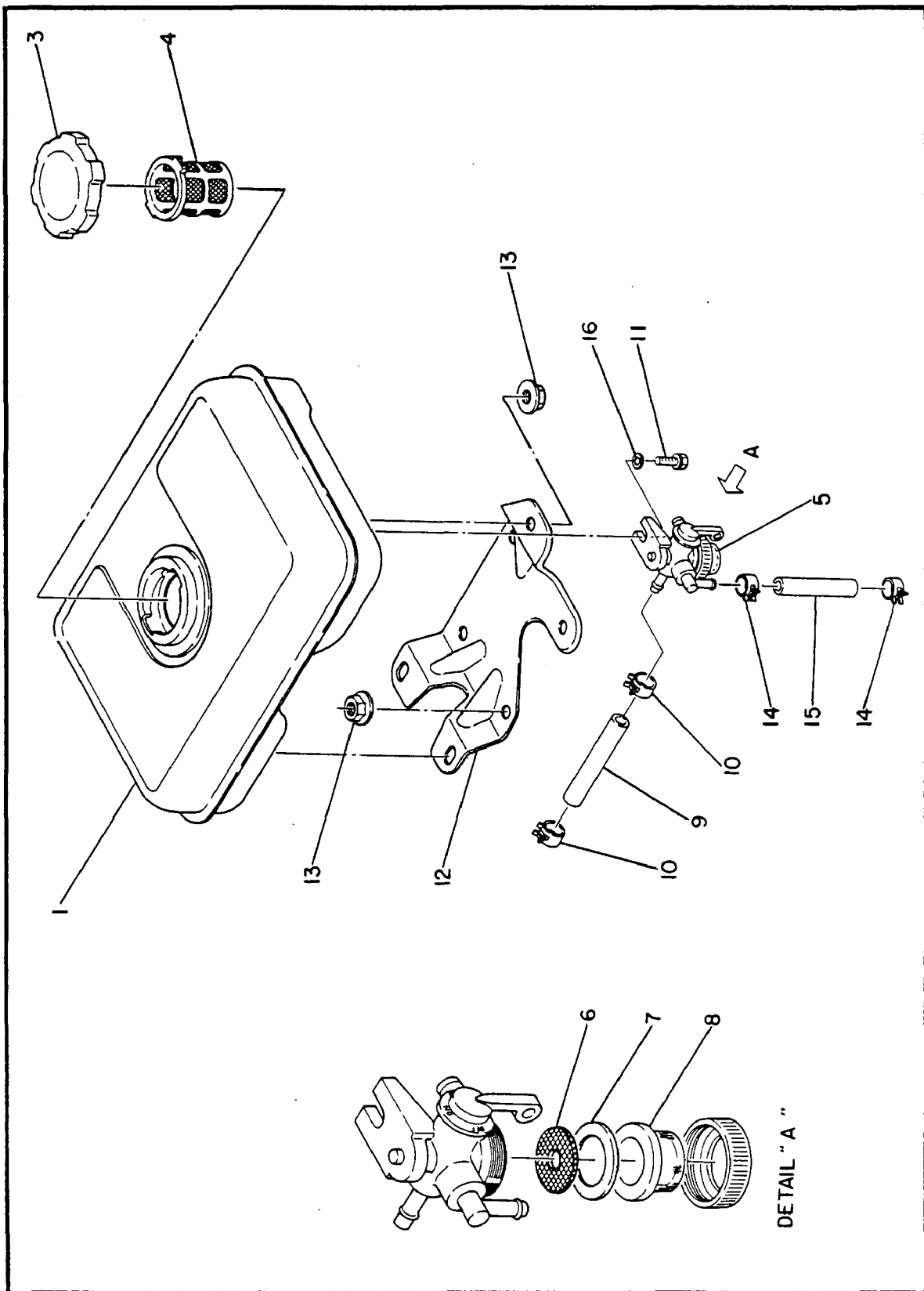
FUEL TANK
