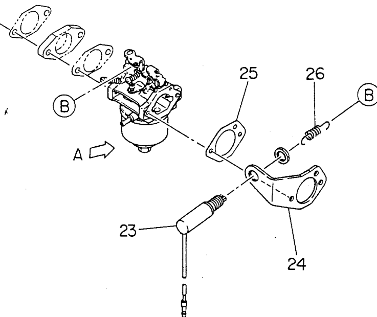
DETAIL "A"
