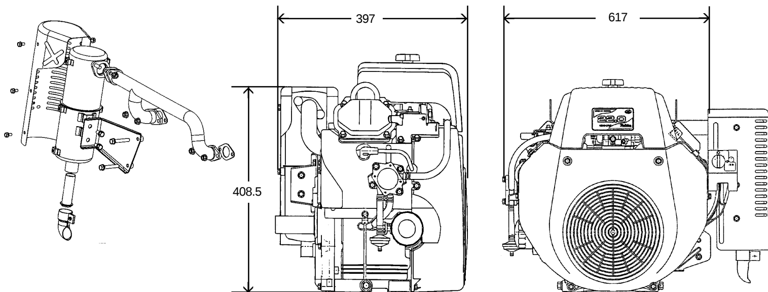
92630020 - Muffler - right side mount
