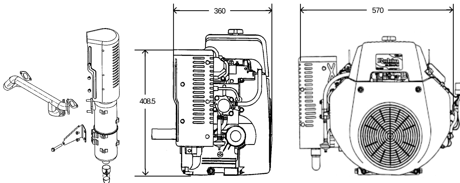
92630034 - Muffler - left side mount, oil filter side
