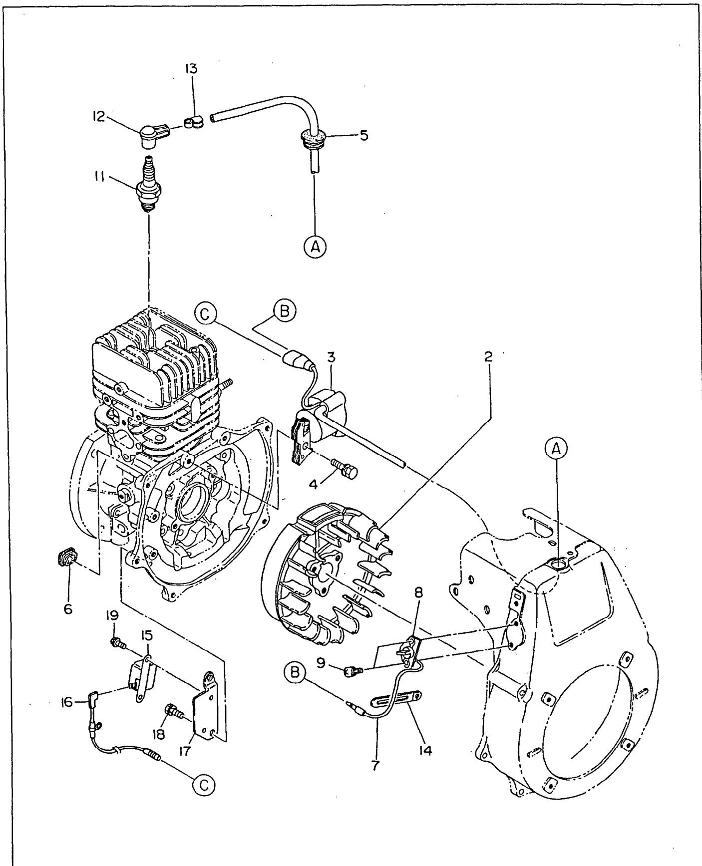
FIG. 5 ELECTRIC DEVICE
